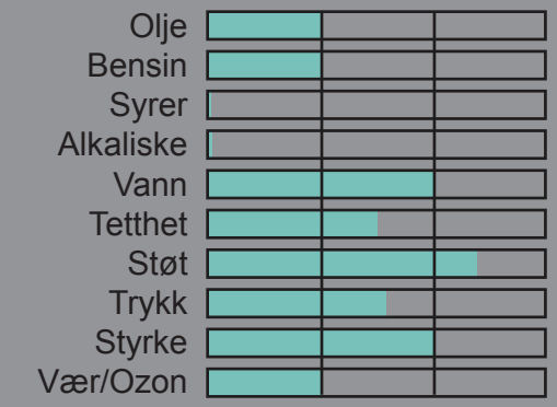
Norsorex (PNR)
