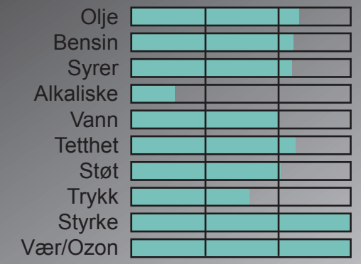
Urethanegummi (AE/EU)
